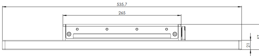
BOTTOM VIEW
