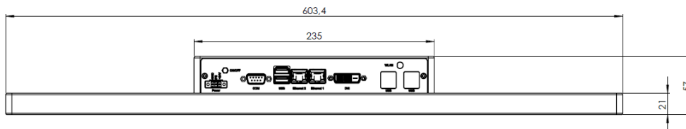
BOTTOM VIEW
