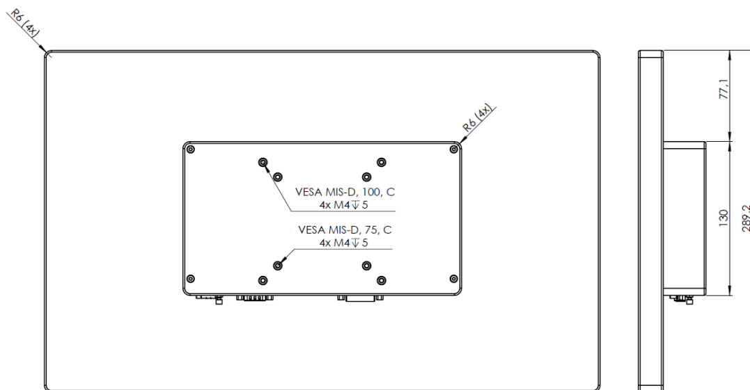
REAR VIEW
