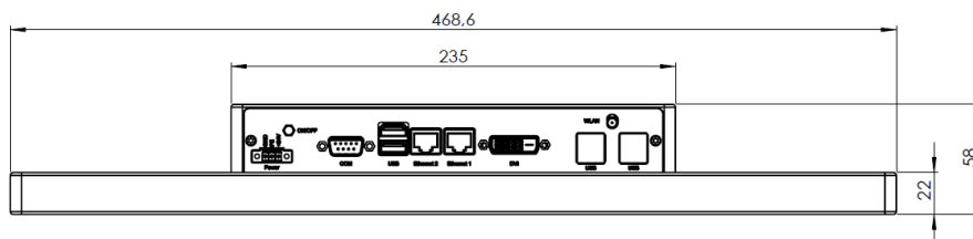
BOTTOM VIEW
