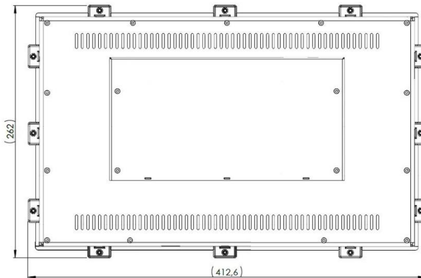
REAR VIEW
