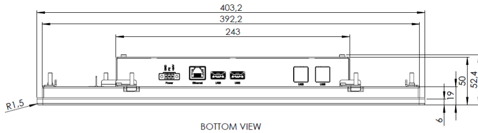
BOTTOM VIEW
