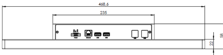
BOTTOM VIEW
