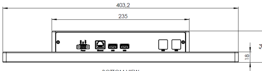
BOTTOM VIEW
