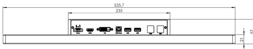
BOTTOM VIEW
