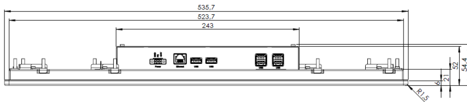
BOTTOM VIEW
